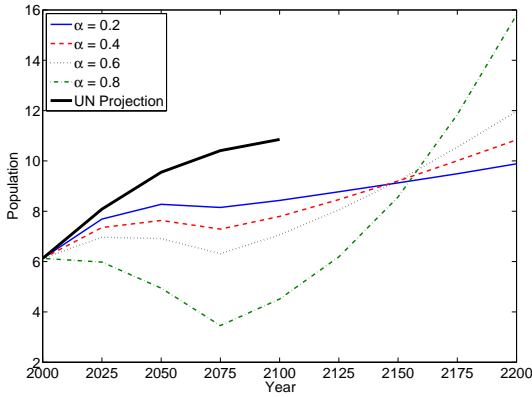
(c) \hat{\beta} = 0.99
