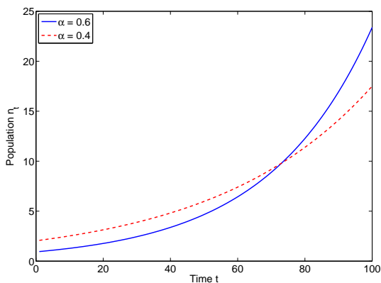
(c) \eta = 0.008
