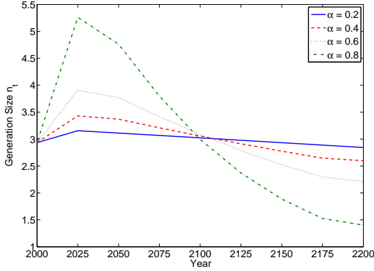
(c) \hat{\beta} = 0.99
