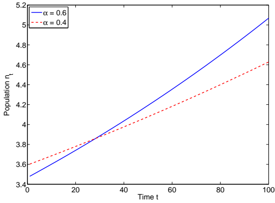
(c) \beta = 0.971
